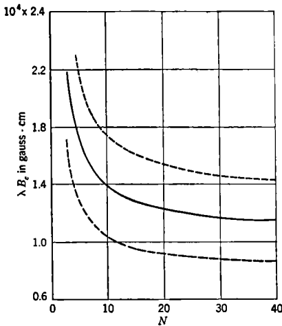
FIG. 10-29.— \lambda B_c as a function of N .
